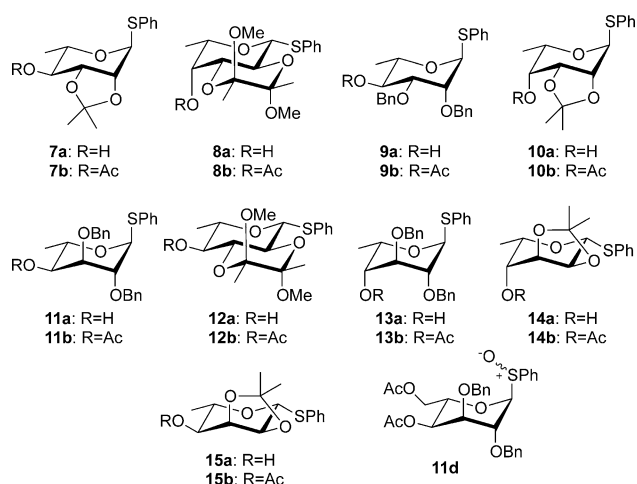
Figure 1. 6-Deoxy L-thio-glycosides used in the synthesis of the L-hexoses, the protodesilylation by-products and the sulfoxide side product 11d.
